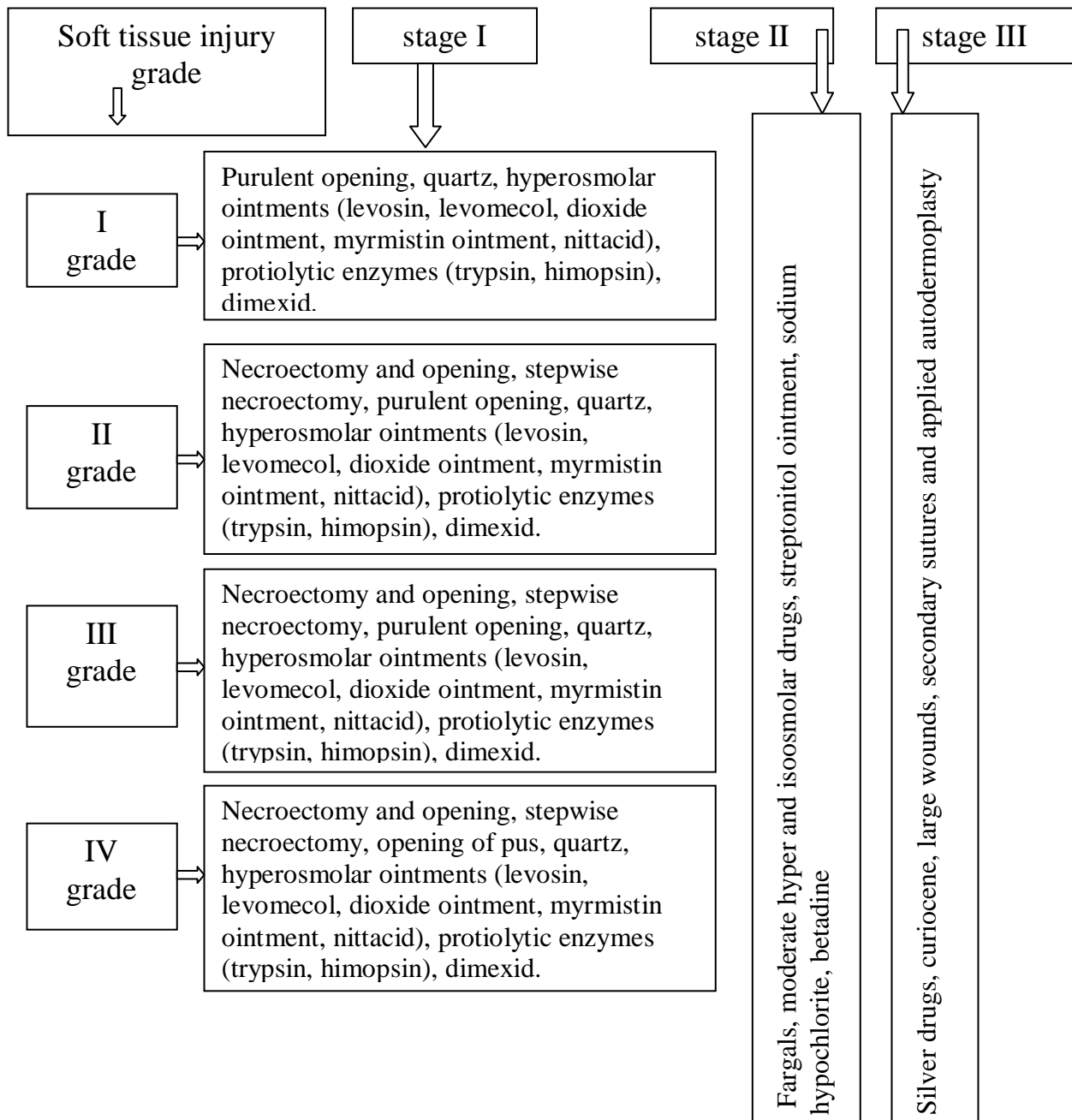
Algorithm for local treatment of wounds.
